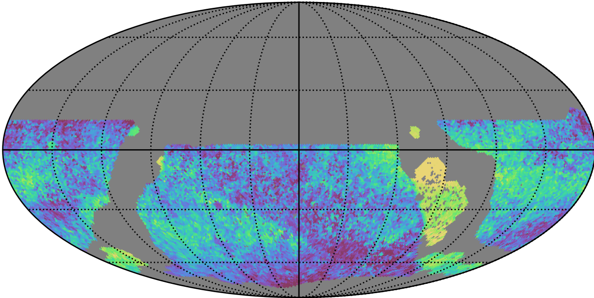
roll_uniform_eh_acc0.2_mjdp0_v3.4_10yrs WFD all bands: Median skyBrightness
