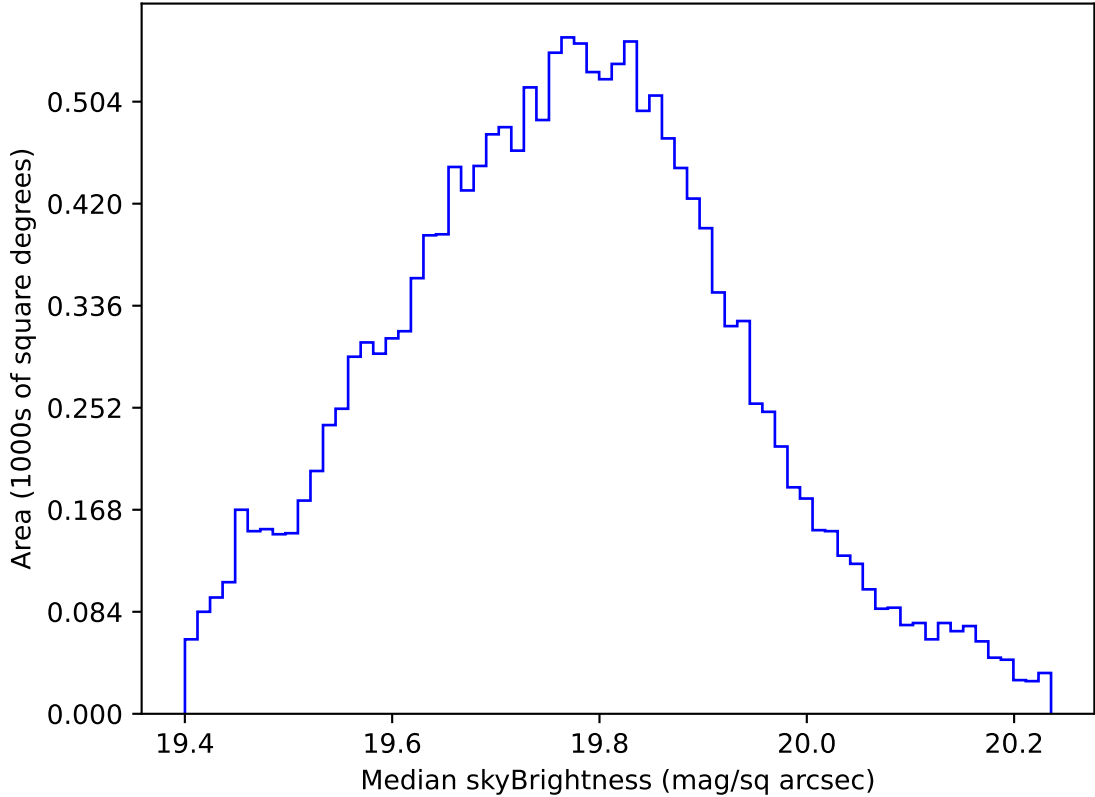
roll_uniform_eh_acc0.2_mjdp0_v3.4_10yrs WFD all bands: Median skyBrightness
