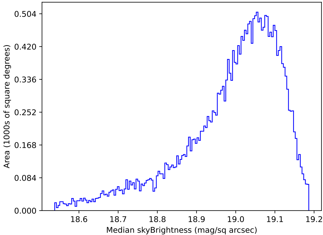
roll_uniform_eh_acc0.2_mjdp0_v3.4_10yrs All sky z band: Median skyBrightness
