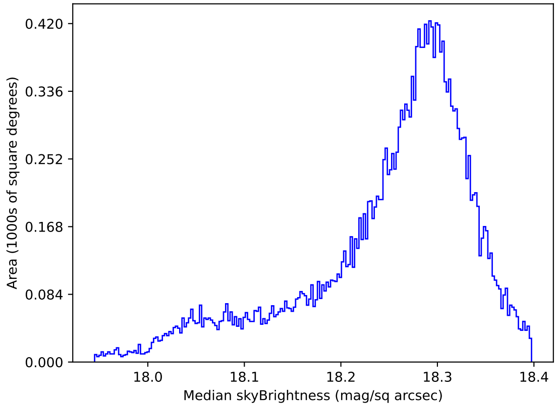
roll_uniform_eh_acc0.2_mjdp0_v3.4_10yrs All sky y band: Median skyBrightness
