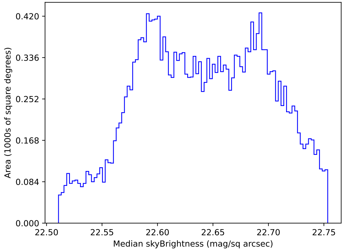
roll_uniform_eh_acc0.2_mjdp0_v3.4_10yrs All sky u band: Median skyBrightness
