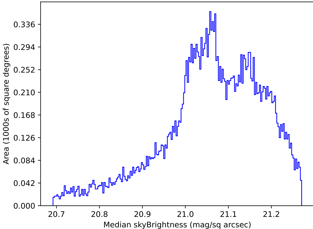
roll_uniform_eh_acc0.2_mjdp0_v3.4_10yrs All sky r band: Median skyBrightness
