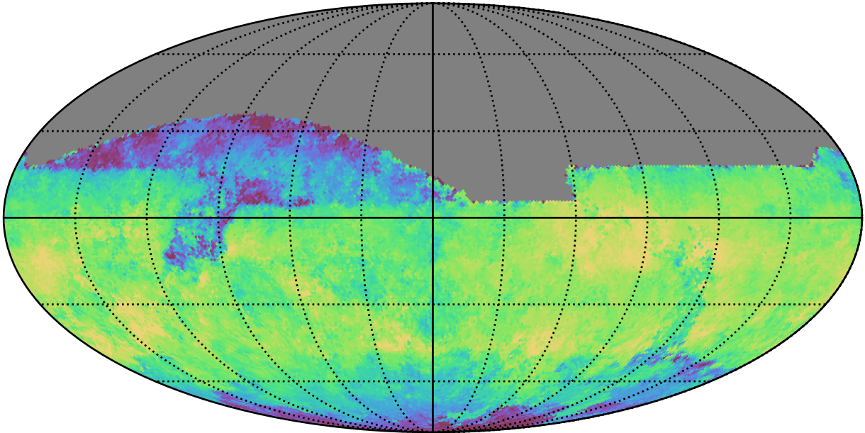
roll_uniform_eh_acc0.2_mjdp0_v3.4_10yrs All sky i band: Median skyBrightness
