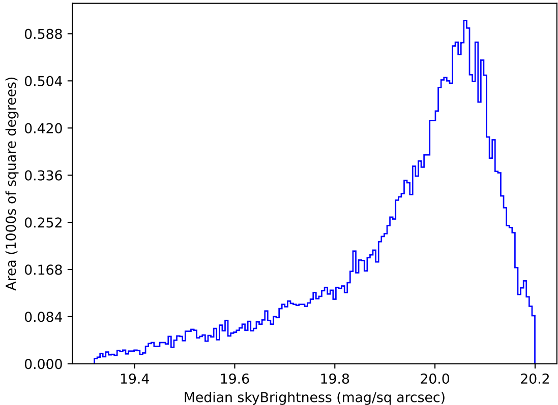
roll_uniform_eh_acc0.2_mjdp0_v3.4_10yrs All sky i band: Median skyBrightness
