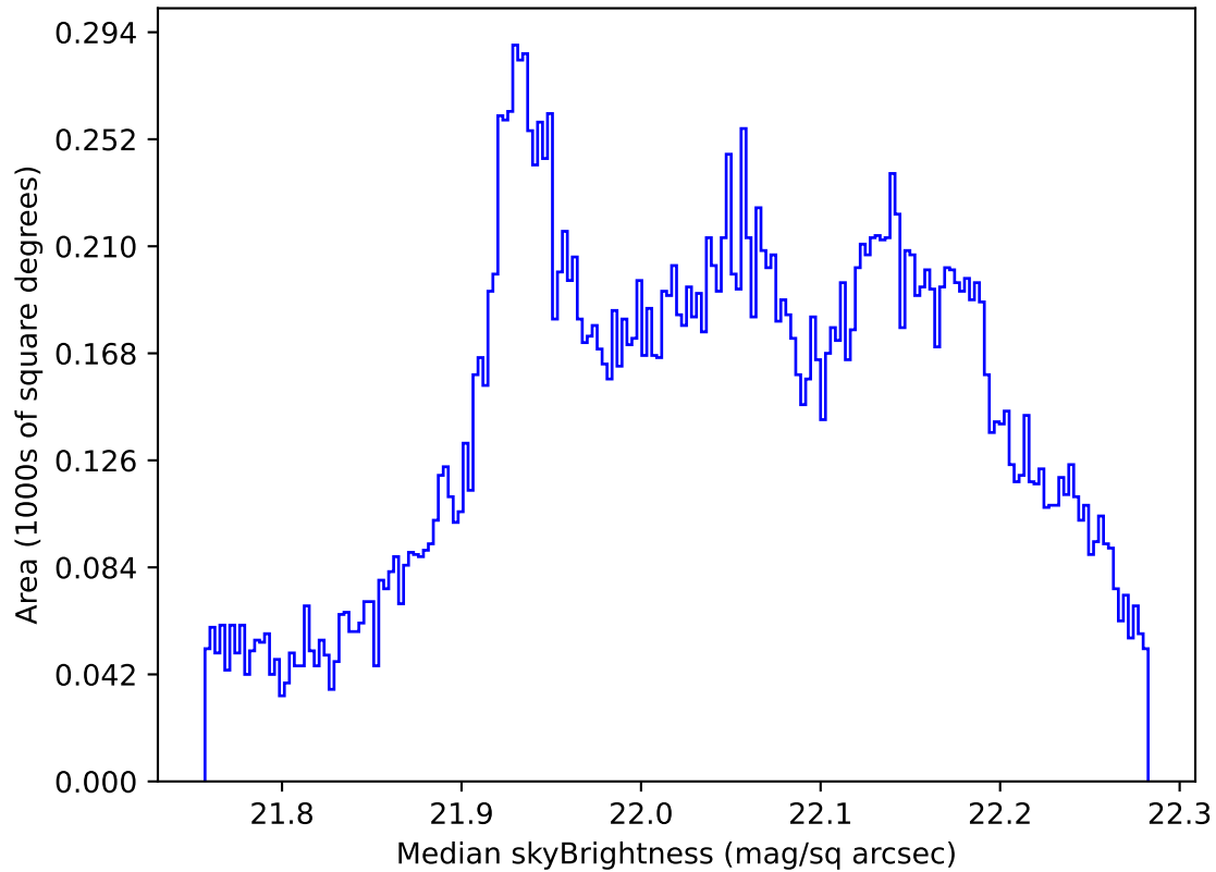
roll_uniform_eh_acc0.2_mjdp0_v3.4_10yrs All sky g band: Median skyBrightness
