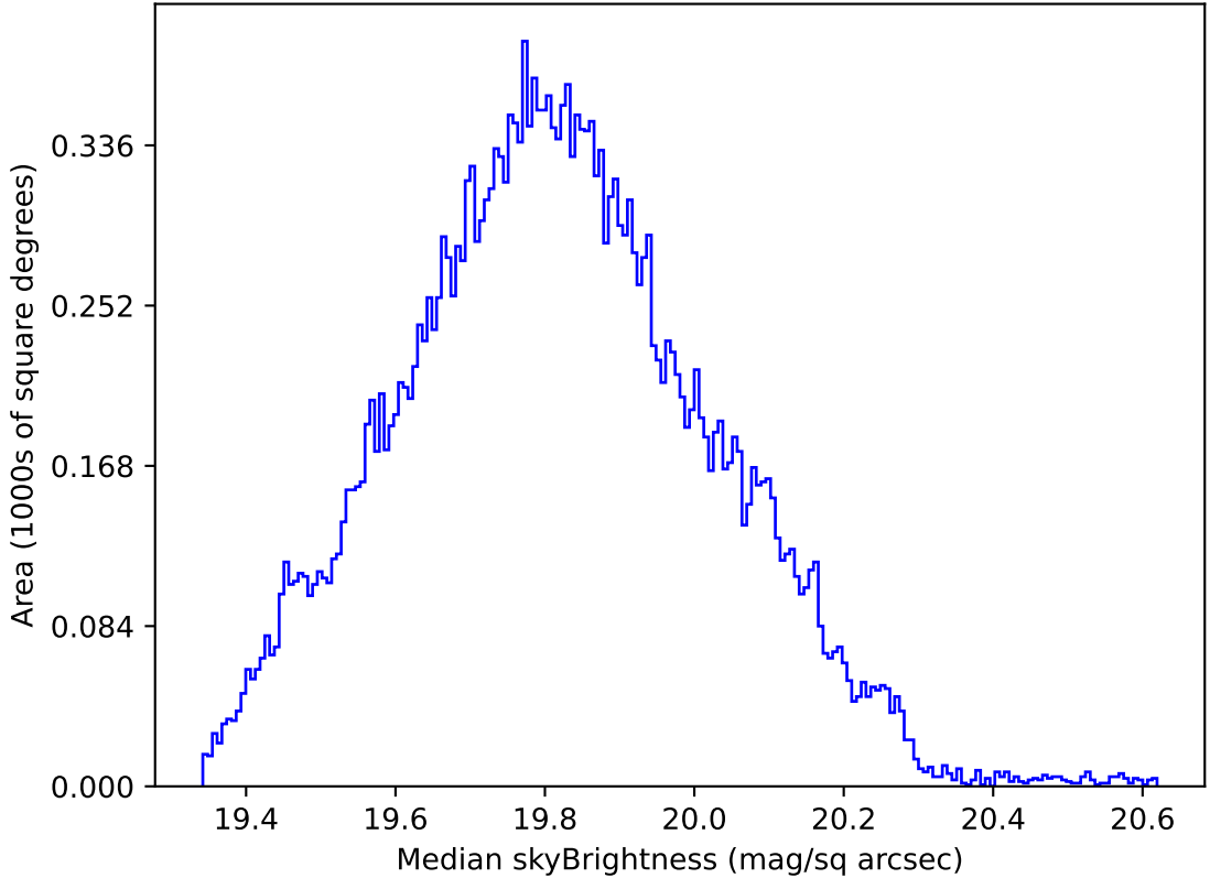
roll_uniform_eh_acc0.2_mjdp0_v3.4_10yrs All sky all bands: Median skyBrightness
