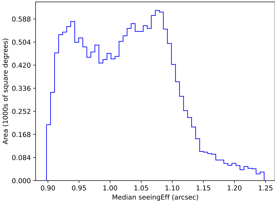
roll_uniform_eh_acc0.2_mjdp0_v3.4_10yrs WFD all bands: Median seeingEff
