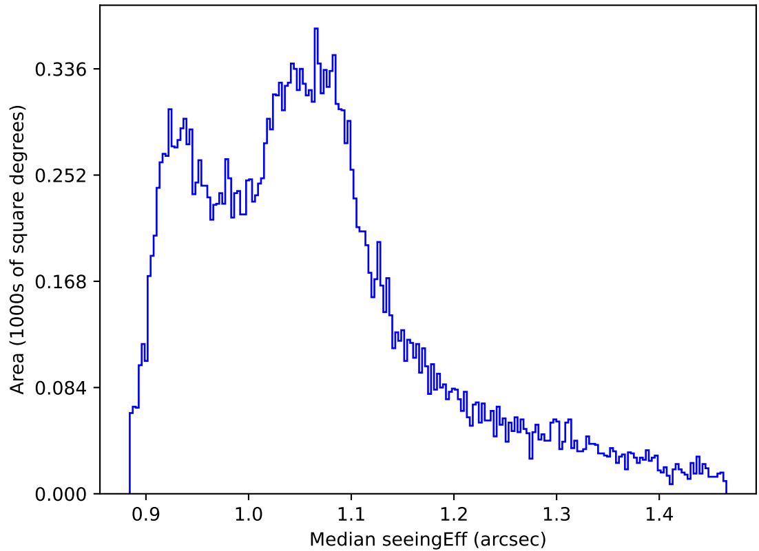
roll_uniform_eh_acc0.2_mjdp0_v3.4_10yrs All sky all bands: Median seeingEff
