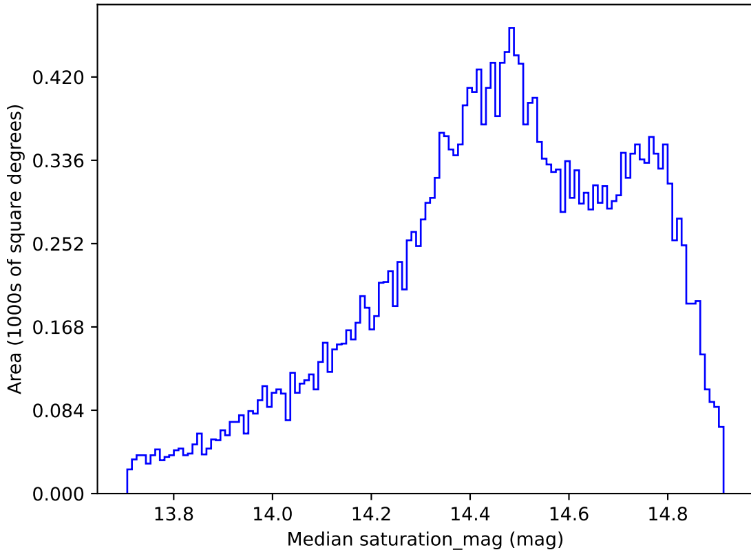
roll_uniform_eh_acc0.2_mjdp0_v3.4_10yrs All sky i band: Median saturation_mag
