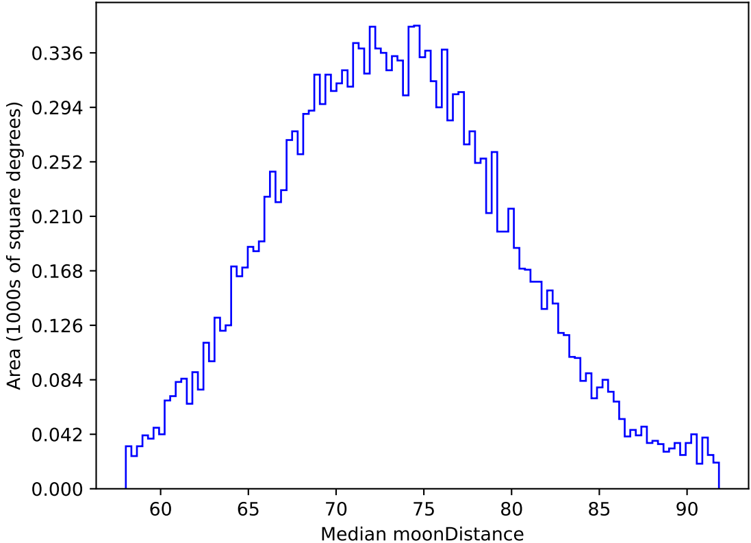
roll_uniform_eh_acc0.2_mjdp0_v3.4_10yrs WFD z band: Median moonDistance
