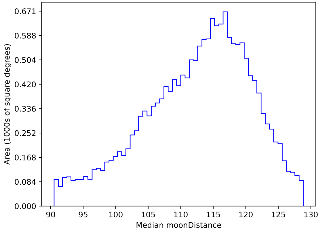
roll_uniform_eh_acc0.2_mjdp0_v3.4_10yrs WFD r band: Median moonDistance
