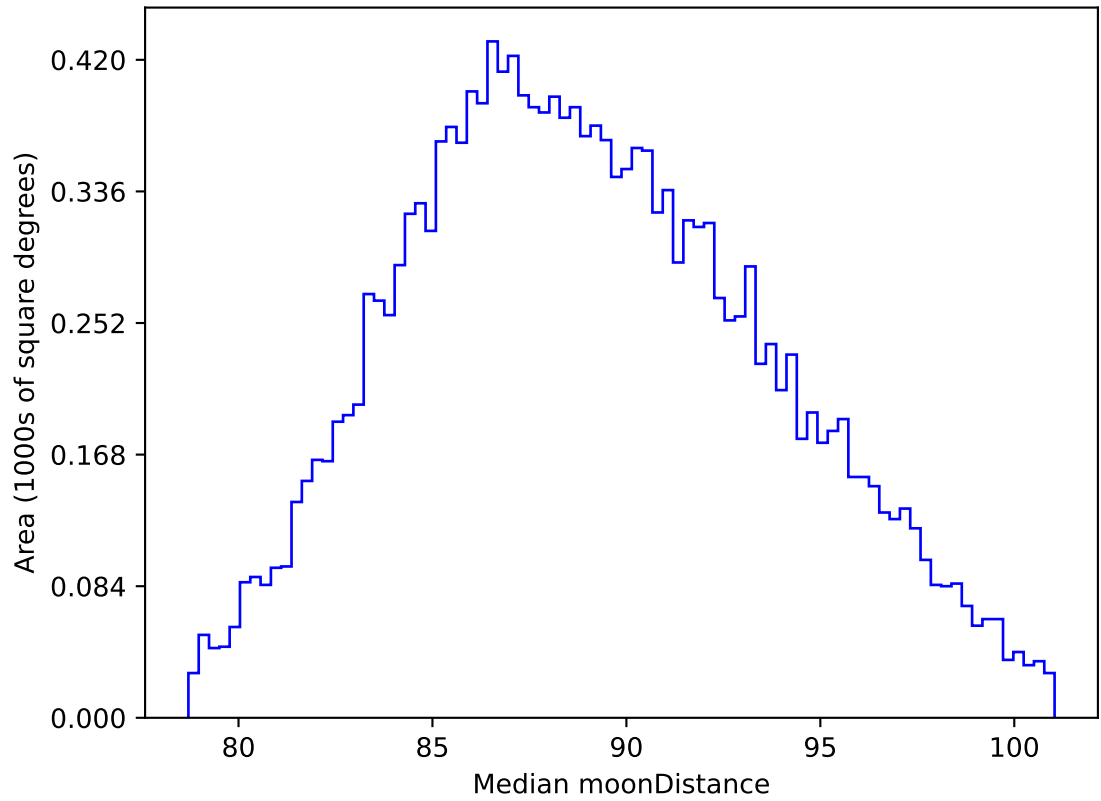
roll_uniform_eh_acc0.2_mjdp0_v3.4_10yrs WFD all bands: Median moonDistance
