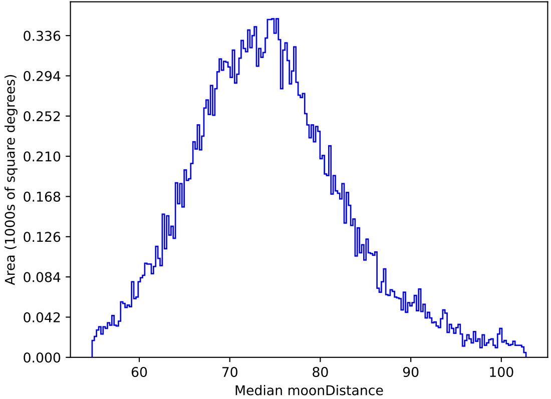
roll_uniform_eh_acc0.2_mjdp0_v3.4_10yrs All sky z band: Median moonDistance
