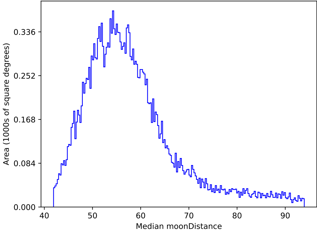
roll_uniform_eh_acc0.2_mjdp0_v3.4_10yrs All sky y band: Median moonDistance
