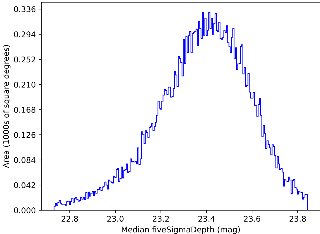
roll_uniform_eh_acc0.2_mjdp0_v3.4_10yrs Yr 1 all bands: Median fiveSigmaDepth
