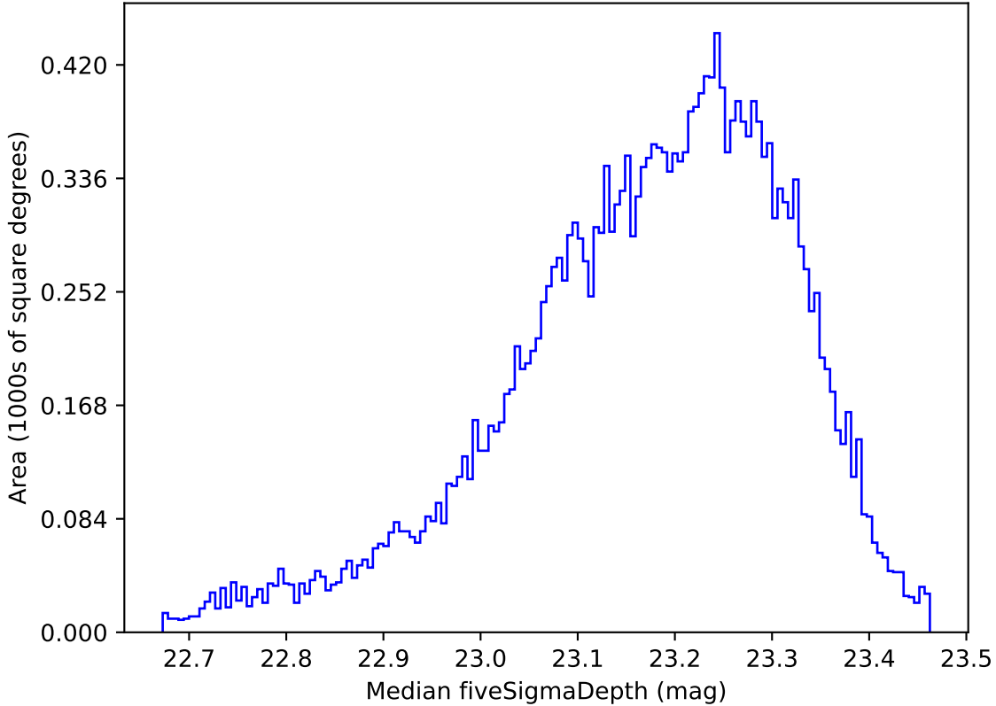
roll_uniform_eh_acc0.2_mjdp0_v3.4_10yrs All sky u band: Median fiveSigmaDepth
