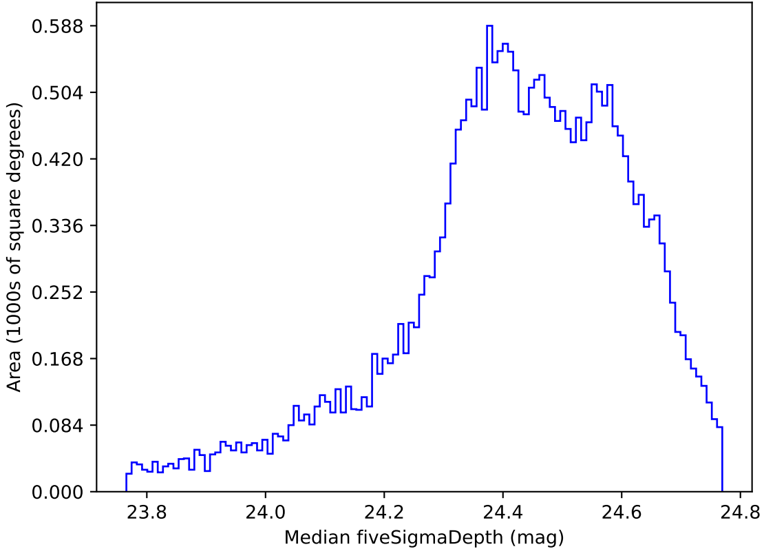
roll_uniform_eh_acc0.2_mjdp0_v3.4_10yrs All sky g band: Median fiveSigmaDepth
