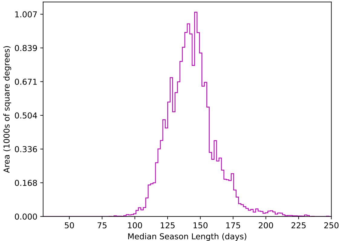
roll_uniform_eh_acc0.2_mjdp0_v3.4_10yrs WFD z band: Median Season Length
