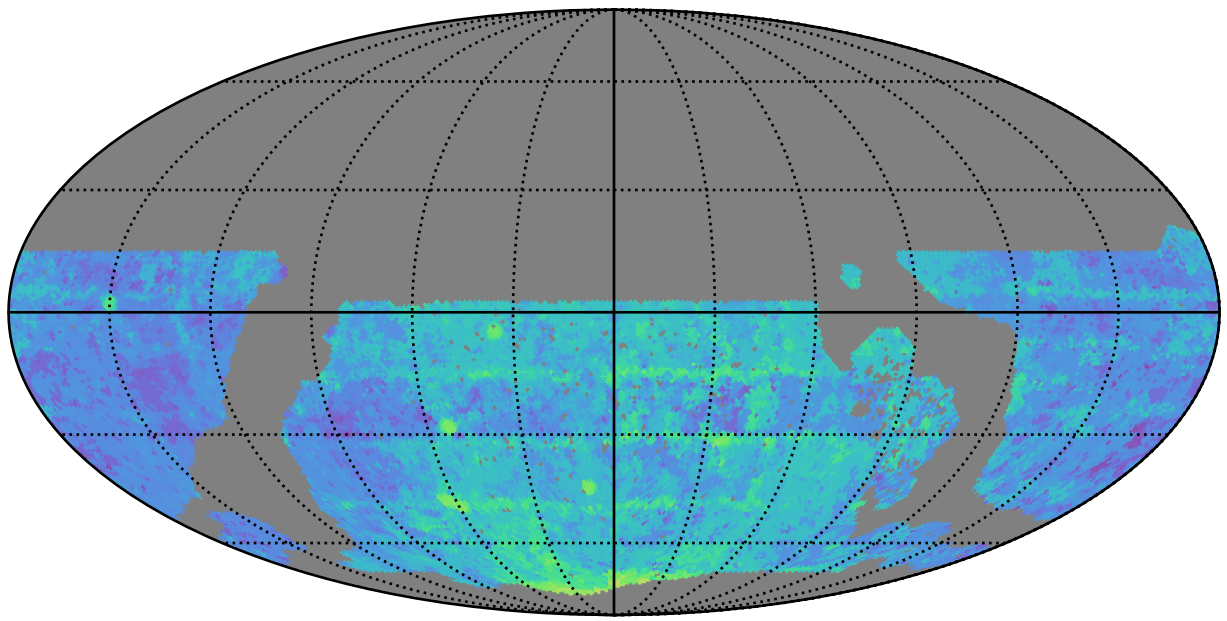
roll_uniform_eh_acc0.2_mjdp0_v3.4_10yrs WFD y band: Median Season Length
