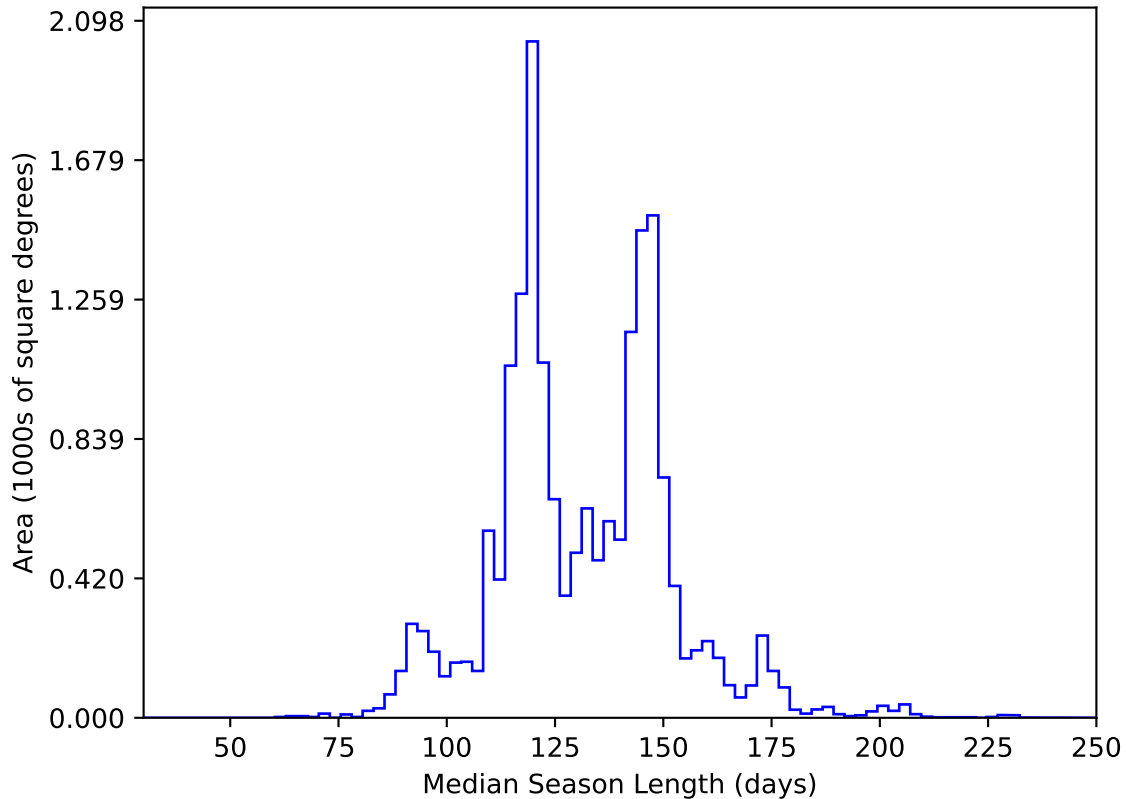
roll_uniform_eh_acc0.2_mjdp0_v3.4_10yrs WFD y band: Median Season Length
