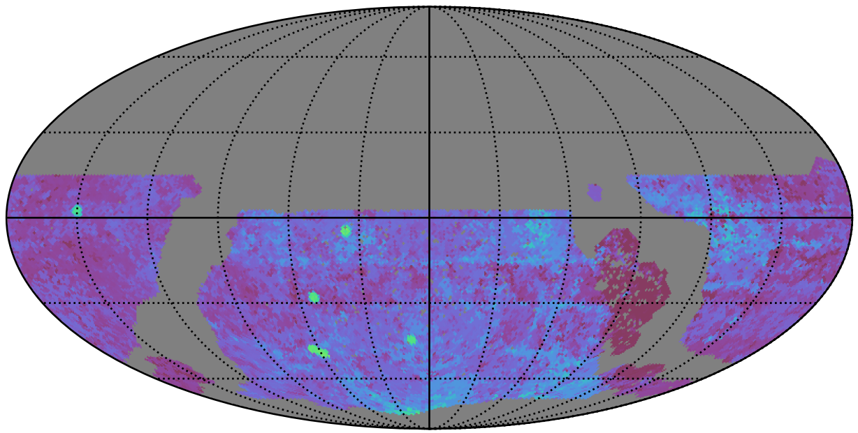
roll_uniform_eh_acc0.2_mjdp0_v3.4_10yrs WFD u band: Median Season Length
