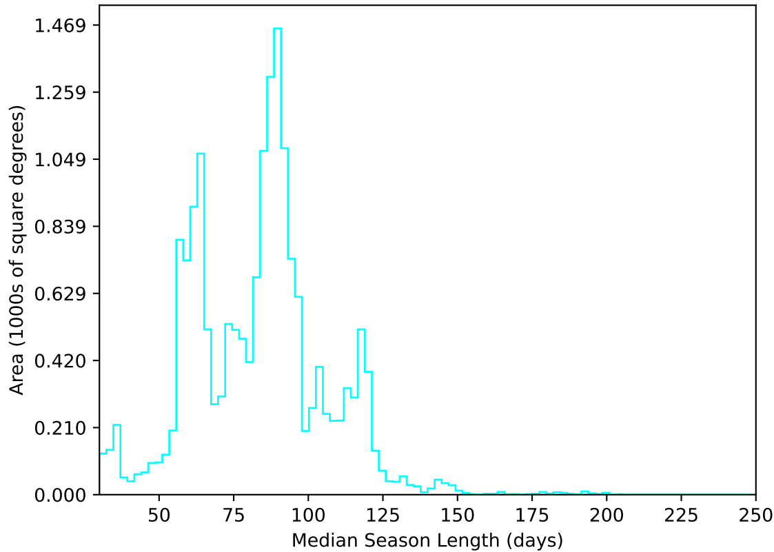
roll_uniform_eh_acc0.2_mjdp0_v3.4_10yrs WFD u band: Median Season Length
