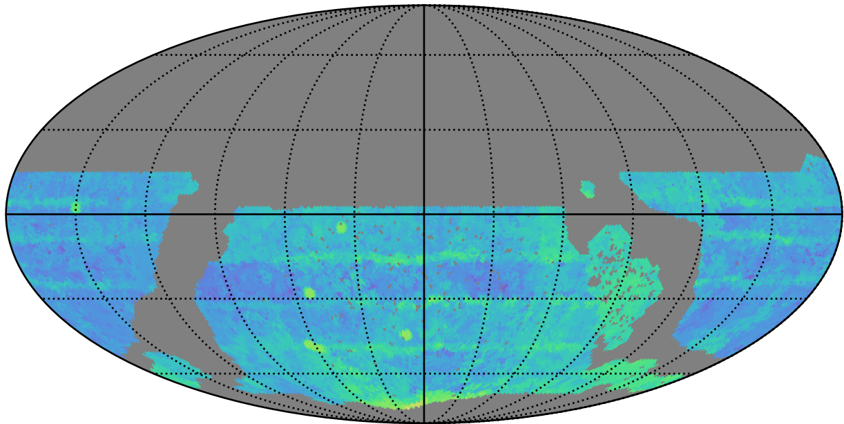
roll_uniform_eh_acc0.2_mjdp0_v3.4_10yrs WFD r band: Median Season Length
