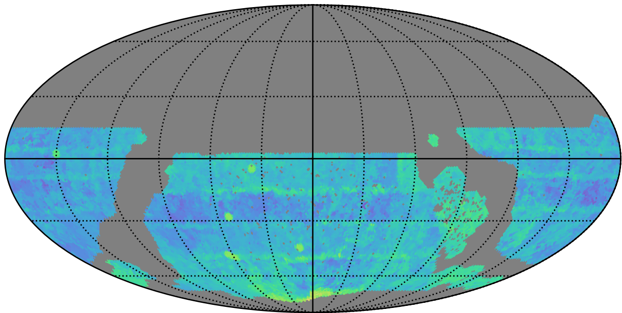
roll_uniform_eh_acc0.2_mjdp0_v3.4_10yrs WFD i band: Median Season Length
