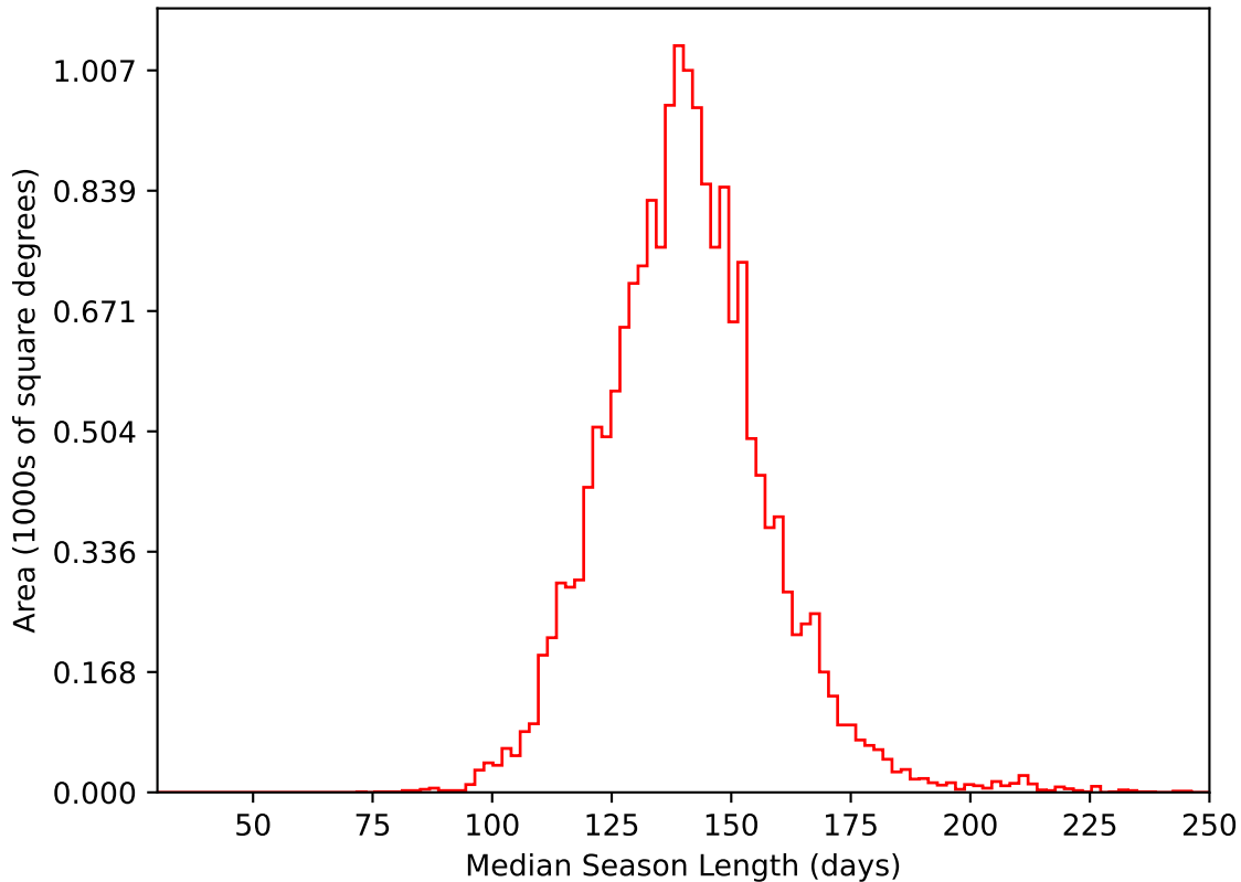
roll_uniform_eh_acc0.2_mjdp0_v3.4_10yrs WFD i band: Median Season Length
