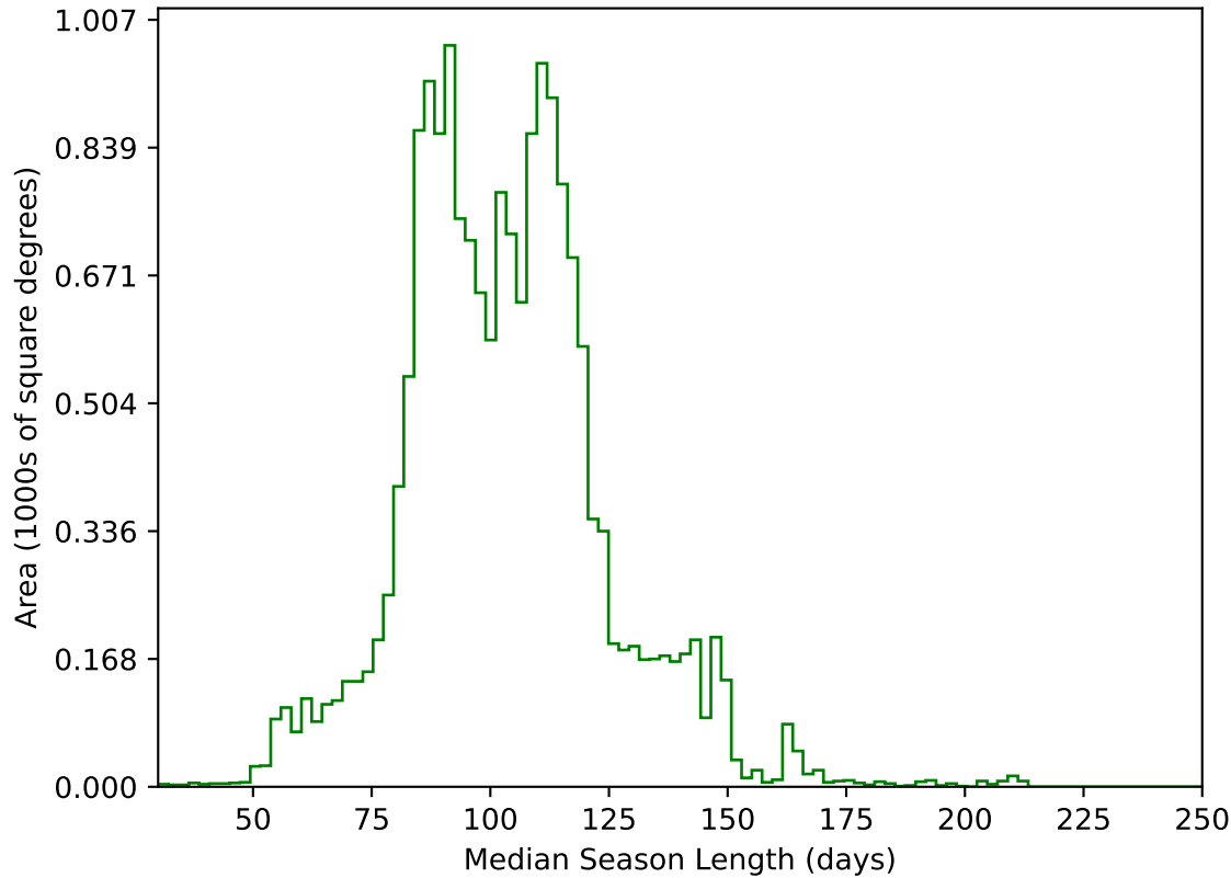
roll_uniform_eh_acc0.2_mjdp0_v3.4_10yrs WFD g band: Median Season Length
