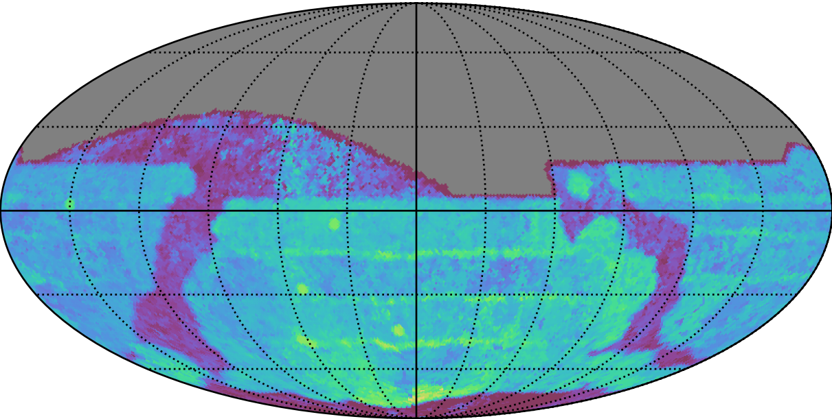
roll_uniform_eh_acc0.2_mjdp0_v3.4_10yrs All sky z band: Median Season Length
