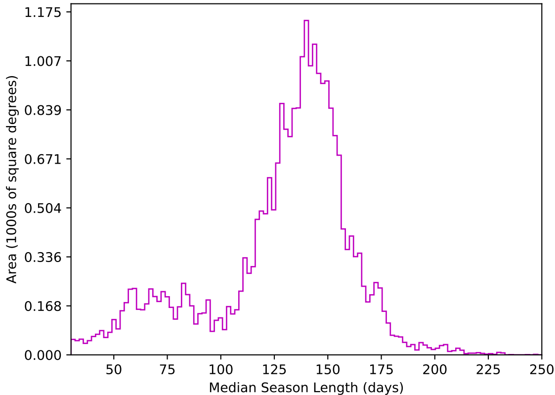
roll_uniform_eh_acc0.2_mjdp0_v3.4_10yrs All sky z band: Median Season Length
