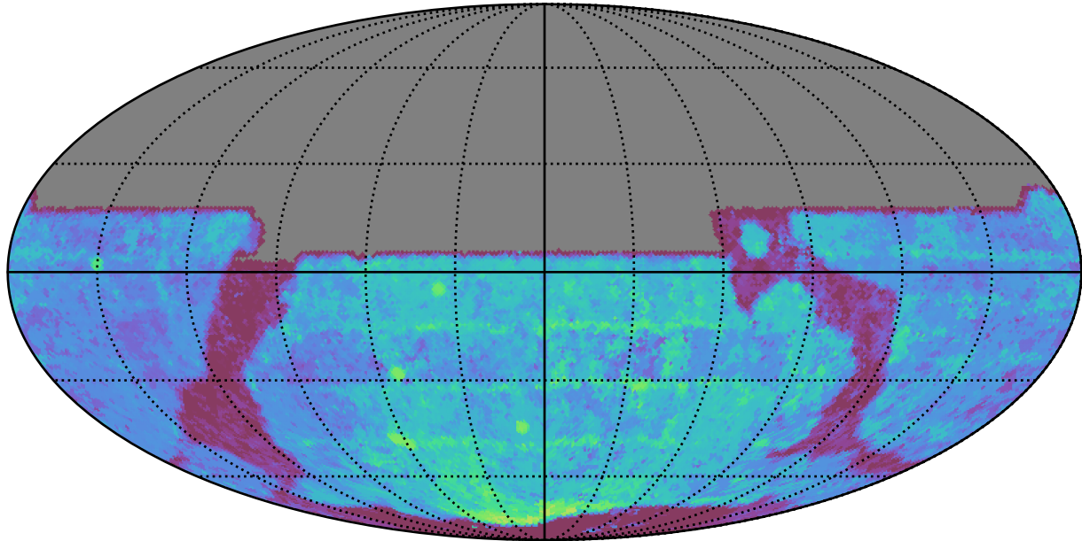
roll_uniform_eh_acc0.2_mjdp0_v3.4_10yrs All sky y band: Median Season Length
