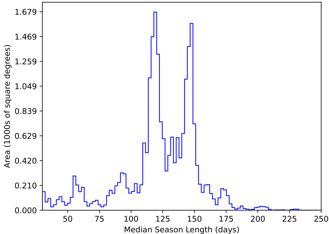
roll_uniform_eh_acc0.2_mjdp0_v3.4_10yrs All sky y band: Median Season Length
