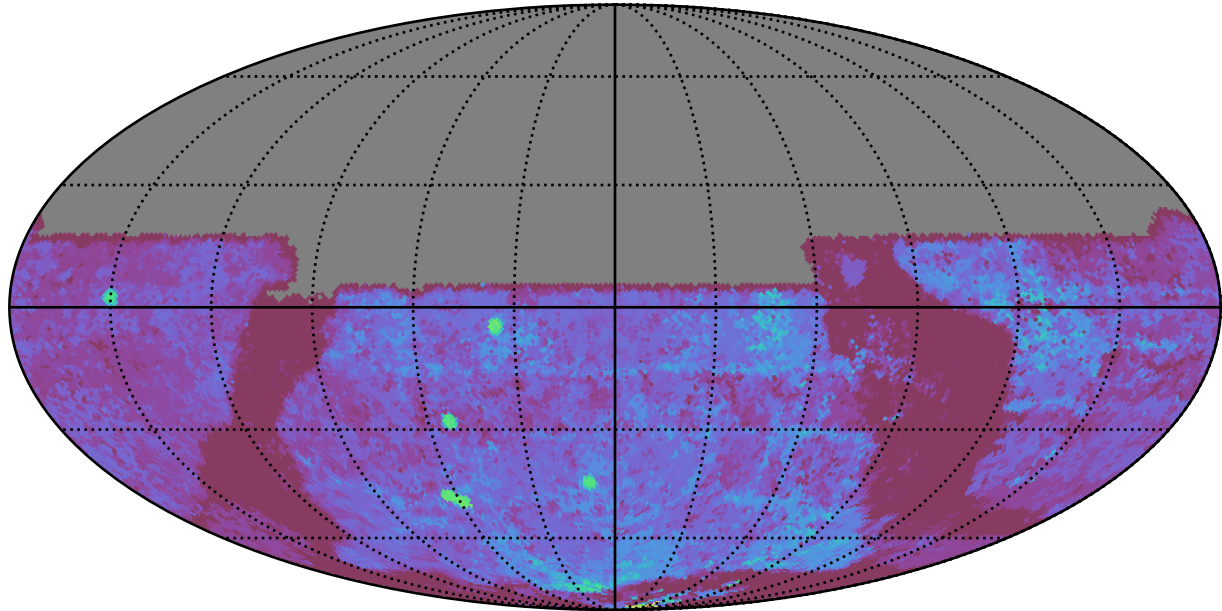
roll_uniform_eh_acc0.2_mjdp0_v3.4_10yrs All sky u band: Median Season Length
