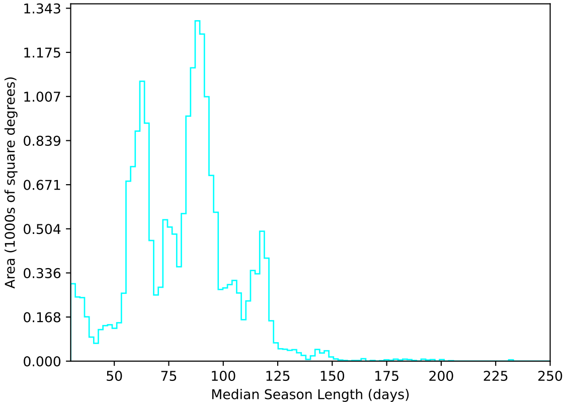
roll_uniform_eh_acc0.2_mjdp0_v3.4_10yrs All sky u band: Median Season Length
