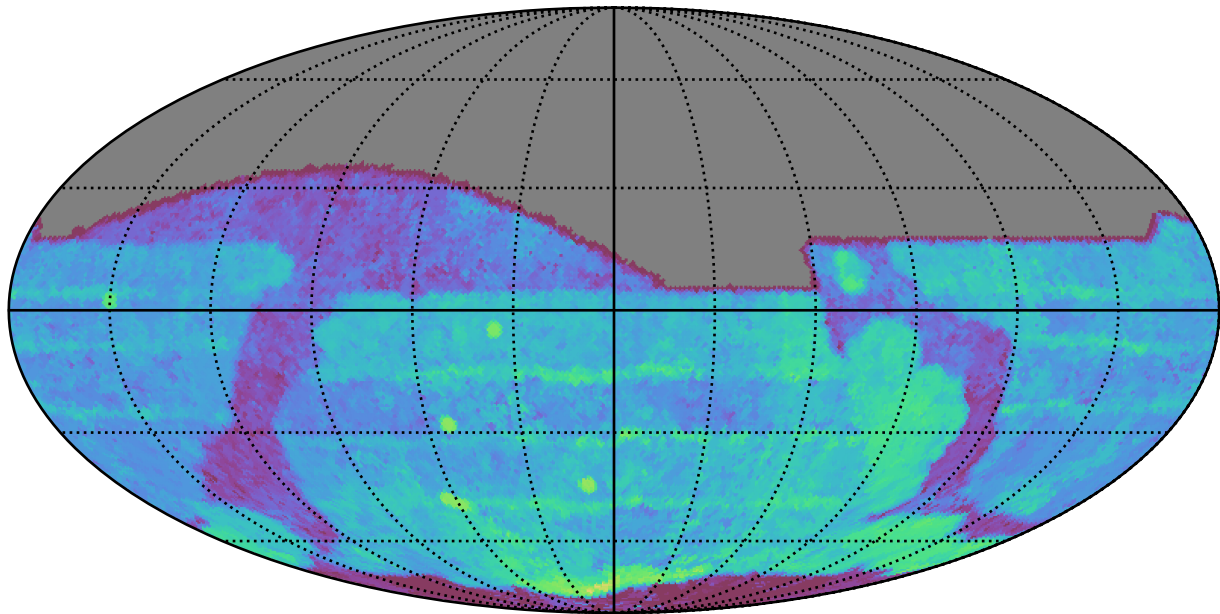
roll_uniform_eh_acc0.2_mjdp0_v3.4_10yrs All sky r band: Median Season Length
