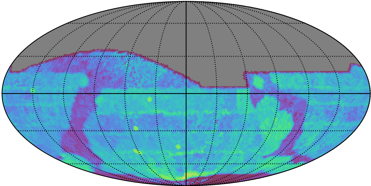
roll_uniform_eh_acc0.2_mjdp0_v3.4_10yrs All sky i band: Median Season Length
