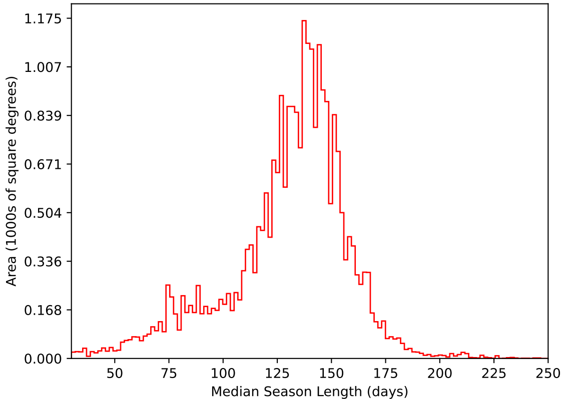
roll_uniform_eh_acc0.2_mjdp0_v3.4_10yrs All sky i band: Median Season Length
