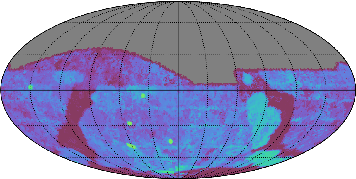
roll_uniform_eh_acc0.2_mjdp0_v3.4_10yrs All sky g band: Median Season Length
