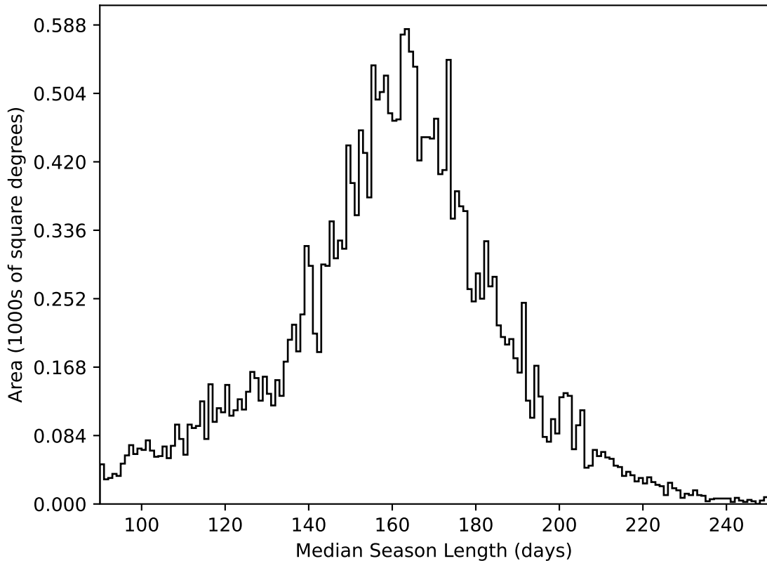
roll_uniform_eh_acc0.2_mjdp0_v3.4_10yrs All sky all bands: Median Season Length
