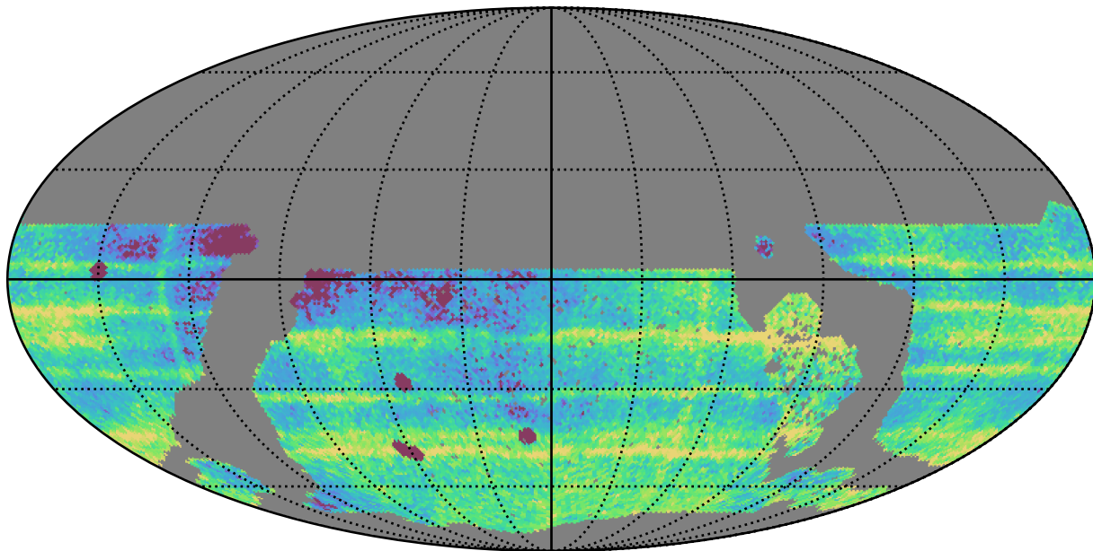
roll_uniform_eh_acc0.2_mjdp0_v3.4_10yrs WFD: Median Intra-Night Gap
