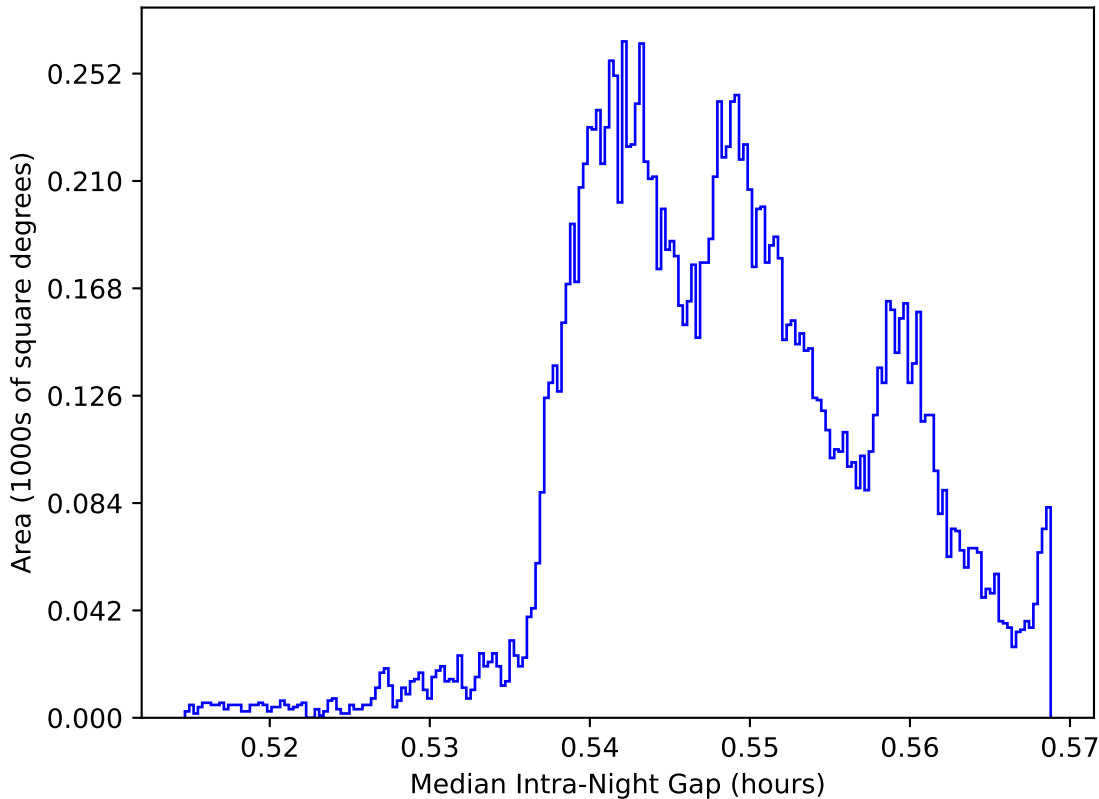
roll_uniform_eh_acc0.2_mjdp0_v3.4_10yrs WFD: Median Intra-Night Gap
