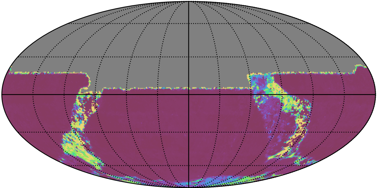
roll_uniform_eh_acc0.2_mjdp0_v3.4_10yrs All sky u band: Median Inter-Night Gap
