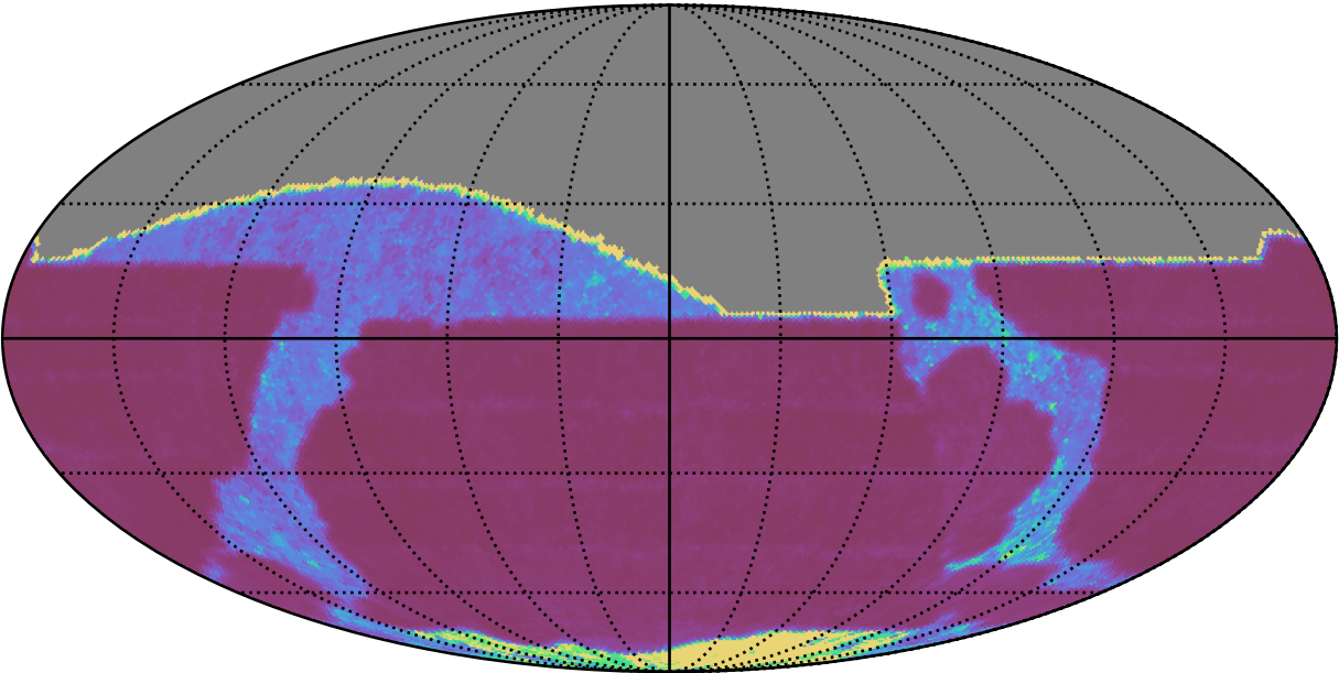
roll_uniform_eh_acc0.2_mjdp0_v3.4_10yrs All sky r band: Median Inter-Night Gap
