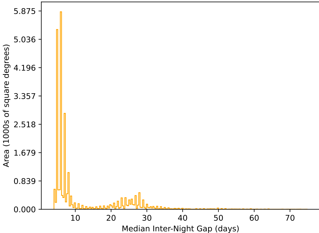
roll_uniform_eh_acc0.2_mjdp0_v3.4_10yrs All sky r band: Median Inter-Night Gap
