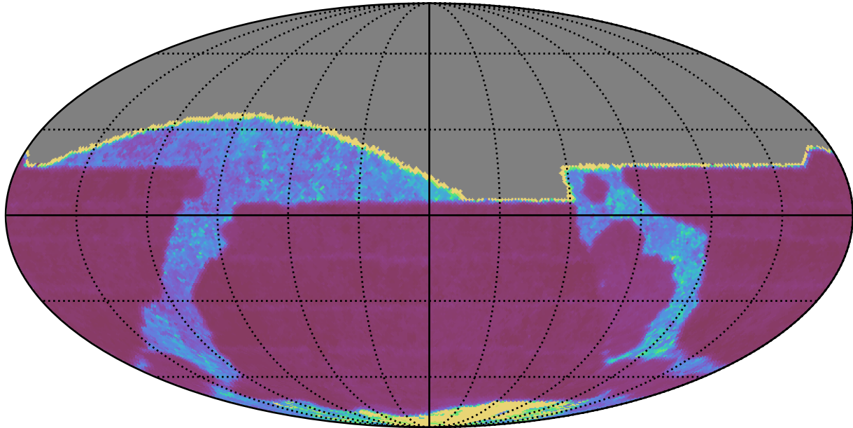
roll_uniform_eh_acc0.2_mjdp0_v3.4_10yrs All sky i band: Median Inter-Night Gap
