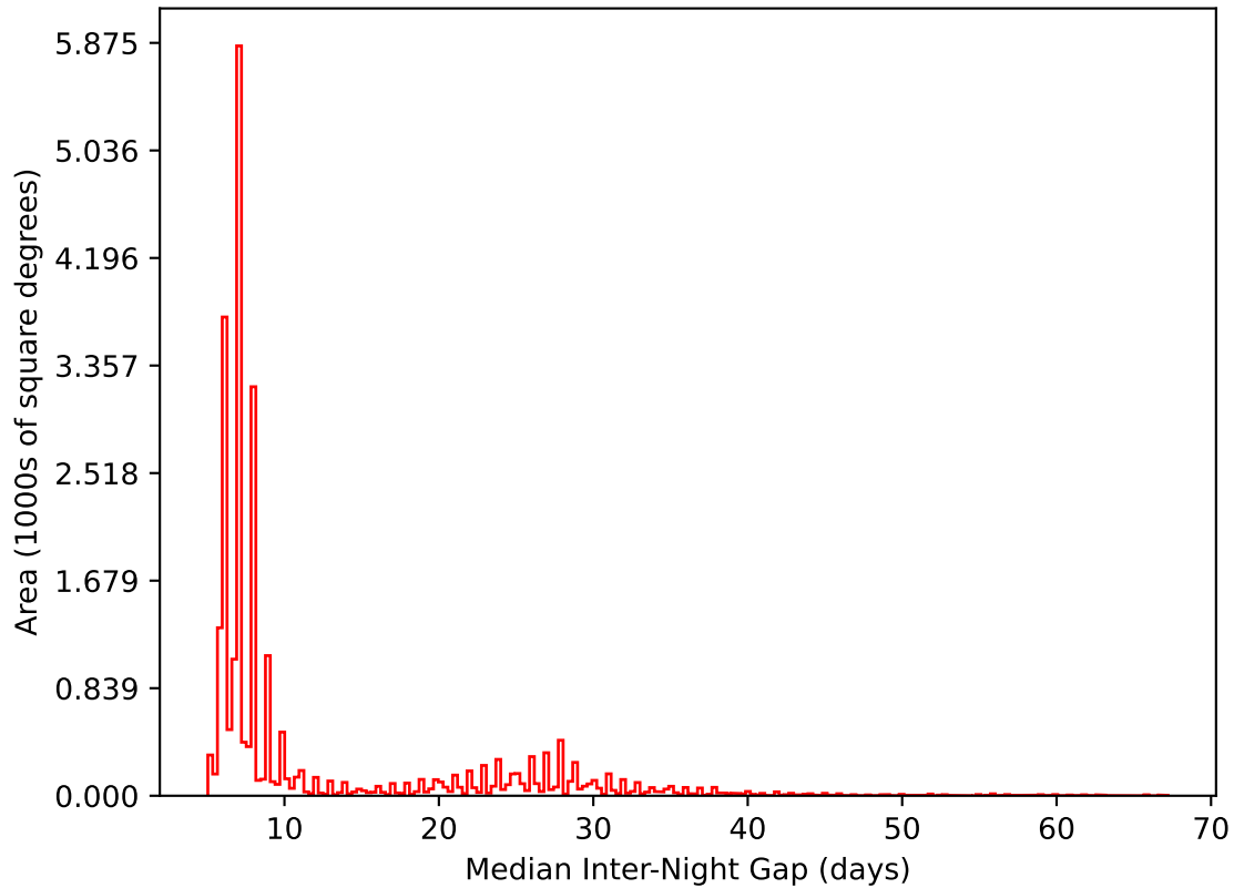
roll_uniform_eh_acc0.2_mjdp0_v3.4_10yrs All sky i band: Median Inter-Night Gap
