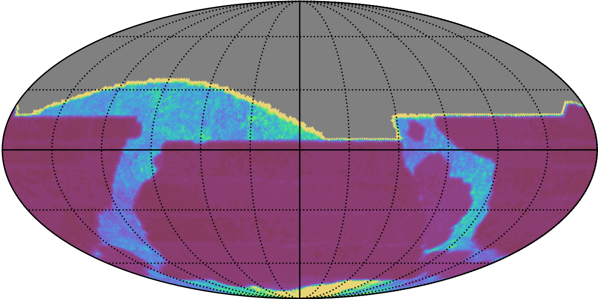
roll_uniform_eh_acc0.2_mjdp0_v3.4_10yrs All sky all bands: Median Inter-Night Gap
