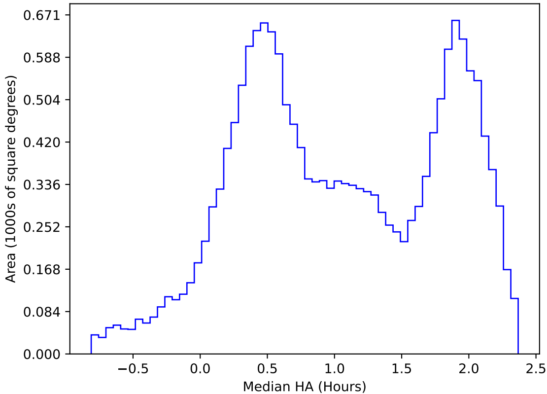
roll_uniform_eh_acc0.2_mjdp0_v3.4_10yrs WFD z band: Median HA
